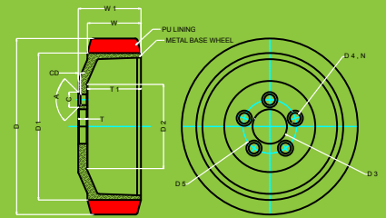
DRIVE WHEEL
