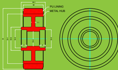
TROLLEY WHEEL
